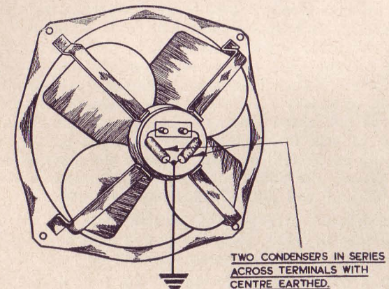
Fig. 14. An improved way of suppressing interference—two condensers in series with the centre earthed.
