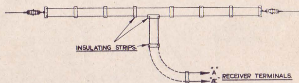
Fig. 5(b). Folded dipole aerial, using ordinary wire and spacing insulators.
